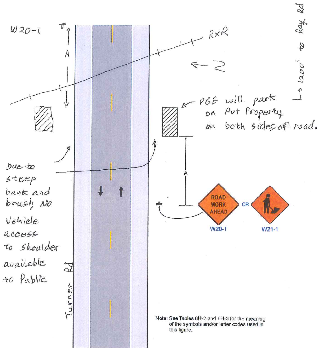
Typical Application 1
